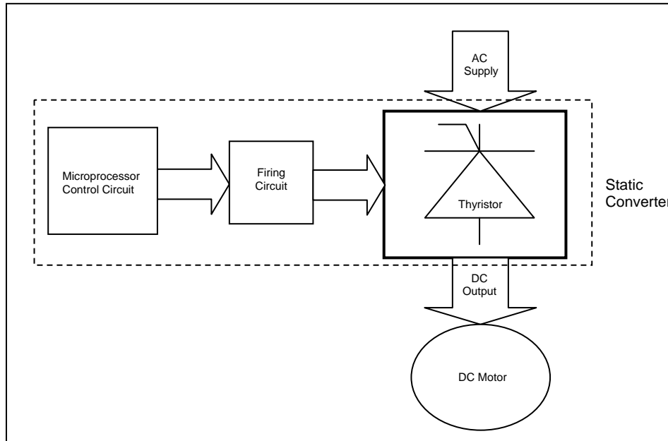
Fig 15: Static converter drive using thyristors fitted with microprocessor control
